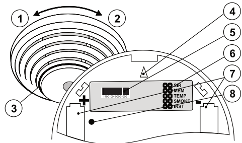
Fig 1: 1 – detector cover opening; 2 – detector cover closing; 3 – optical status signalling; 4 – arrow showing where to insert the detector; 5 – production code; 6 – configuration terminals; 7 – battery holders; 8 – button for test
